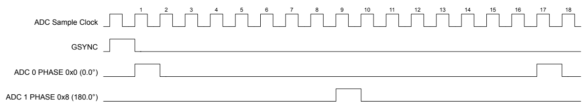
Figure 12-4. Doubling the ADC Sample Rate
